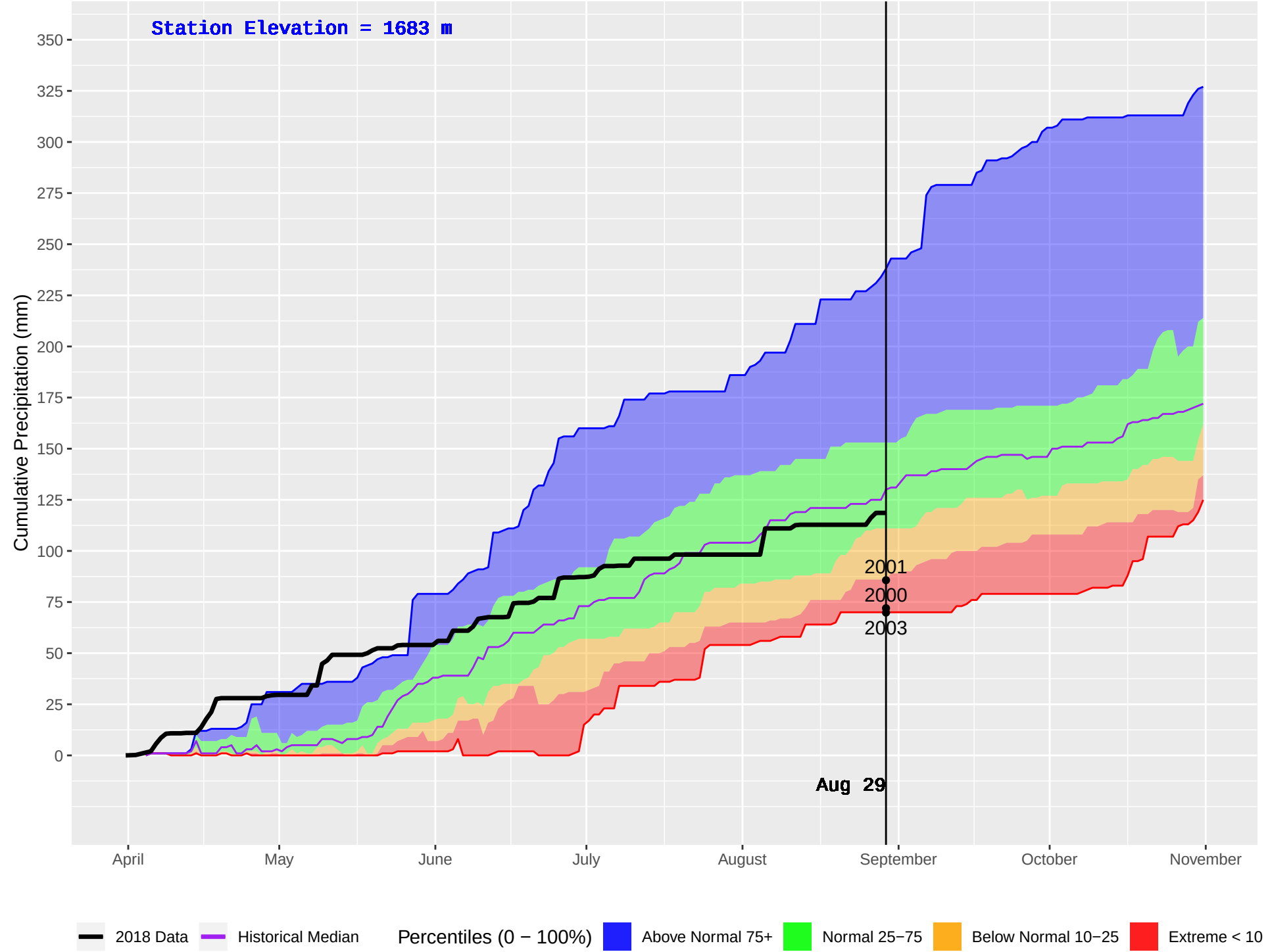
ASHNOLA (331) : Historical (1992–2016) and Current (2018) Daily Cumulative Precipitation
