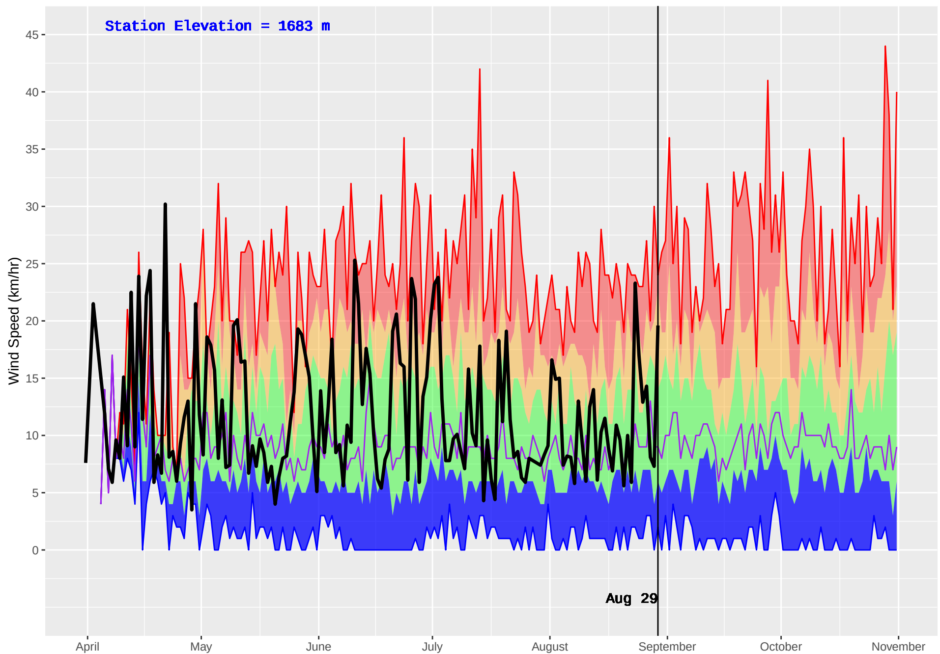
ASHNOLA (331) : Historical (1992–2016) and Current (2018) Daily Wind Speed
